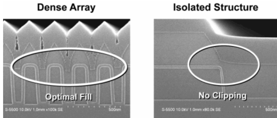
Figure 2: SPEED Max SPM-F process optimized for 32 nm.
