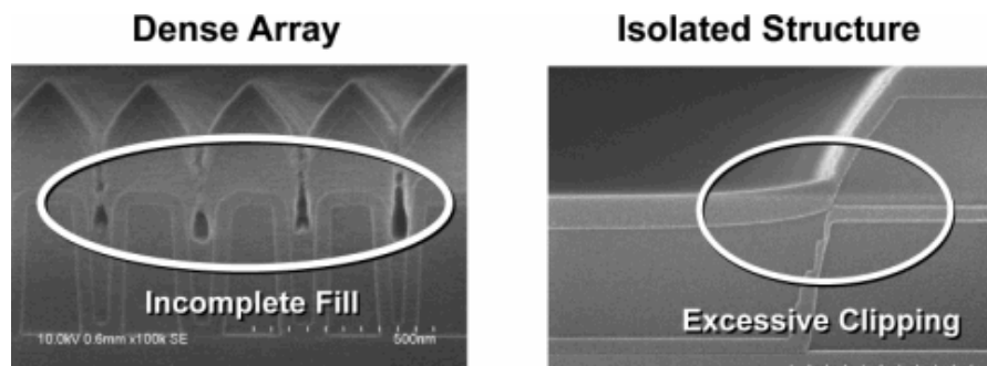
Figure 1: 32 nm baseline process with incomplete fill and excessive clipping.
